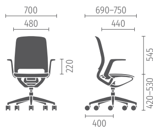
Fixe Armlehnen (standard)
